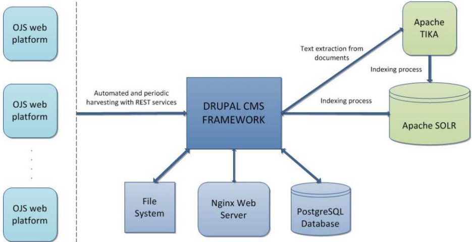
Figure 1: EKT ePublishing platform architecture.
